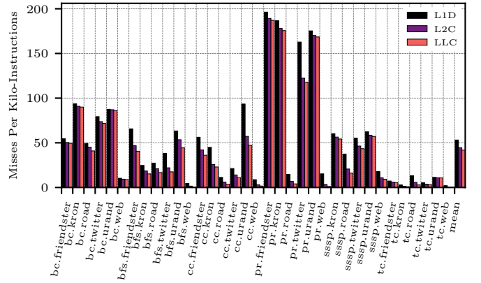
Fig. 2. Misses-Per-Kilo-Instruction (MPKI) across the different levels of the cache hierarchy triggered by graph-processing workloads.
