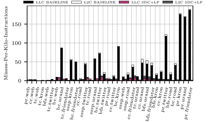
Fig. 8. MPKI of L2C and LLC relatively to theirs counterparts in the baseline.
