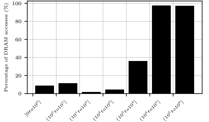
Fig. 3. Probability of accessing DRAM for accesses exhibiting different strides. Data corresponds to the cc.friendster workload.
